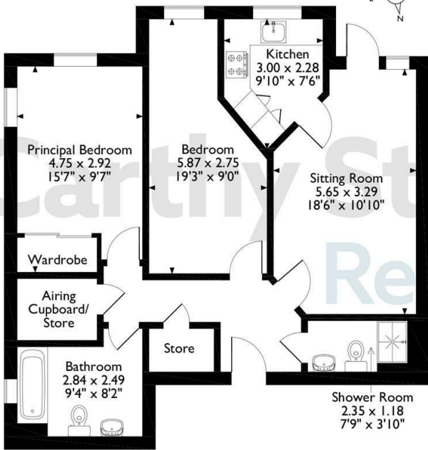
Ground Floor Flat The position & size of doors, windows, appliances and other features are approximate only. © ehouse. Unauthorised reproduction prohibited. Drawing ref. dig/8640736/DST.
